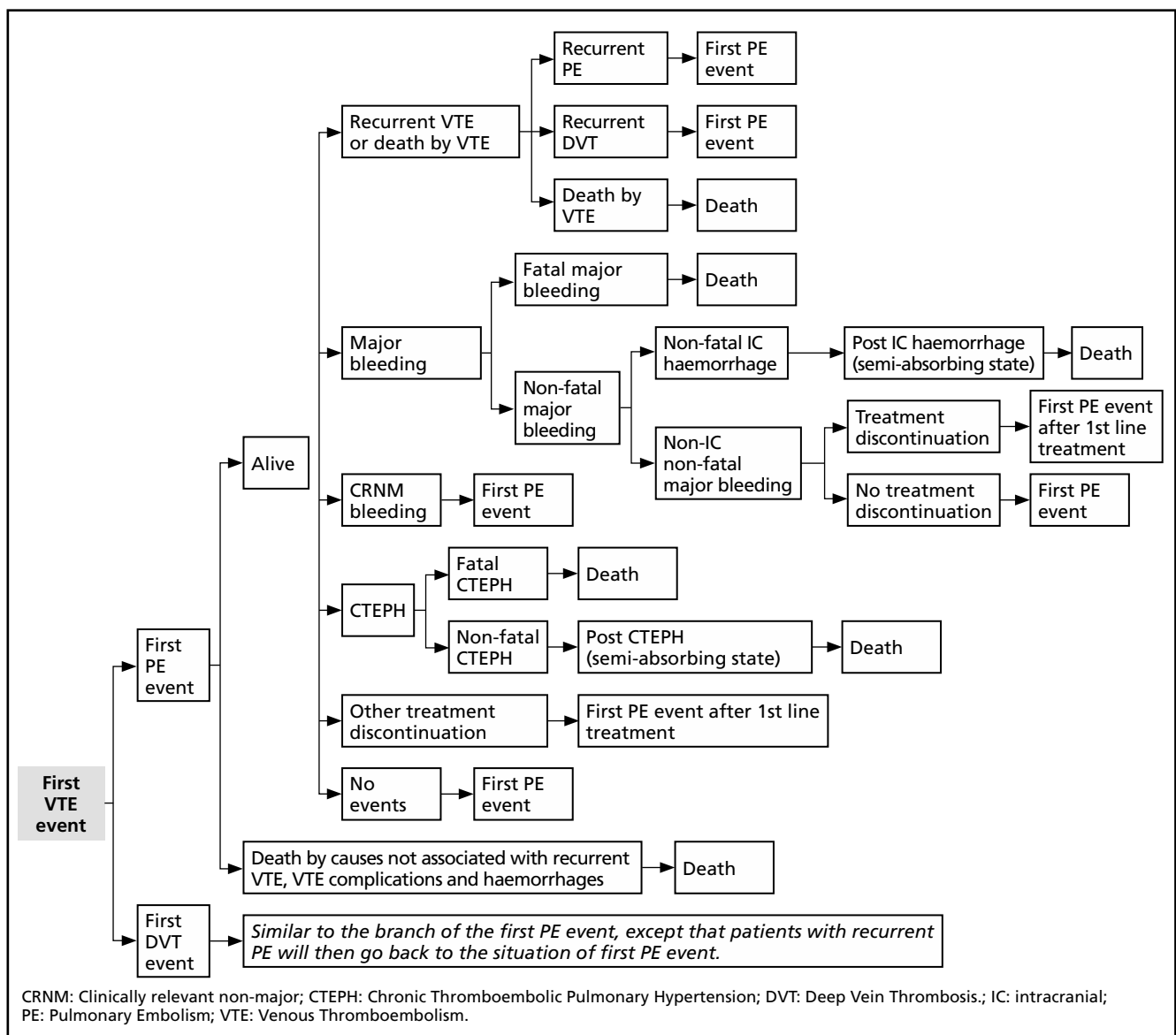
Figure 1. Markov Model.
